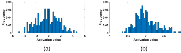
Figure 10: Distribution of the activation maps for (a) marked and (b) unmarked models. DeepSigns preserves the intrinsic distribution while securely embedding the WM information. WM key is generated based on i.i.d. random distribution. If the WM is embedded in hidden layers, the search space for the attacker to find WM keys is \mathcal{O}(\prod_{l \in L} \binom{S_l}{s_l} R^{M_l \times N_l}) . Here, L is the set of hidden layers used for watermarking, s_l , M_l and N_l denote the number of WM-related Gaussian centers, the dimension of activation maps, and the length of the WM signature in the l^{th} layer, respectively. R is the number of values in the domain used for creating projection matrix A ( A \in \mathbb{R} so R is infinity).
