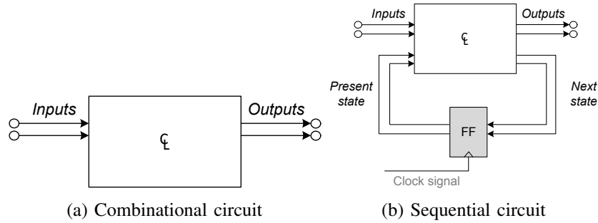
Fig. 3: (a) Combinational circuit where outputs are functions of only inputs. (b) Sequential circuit where outputs are functions of inputs and present states.
