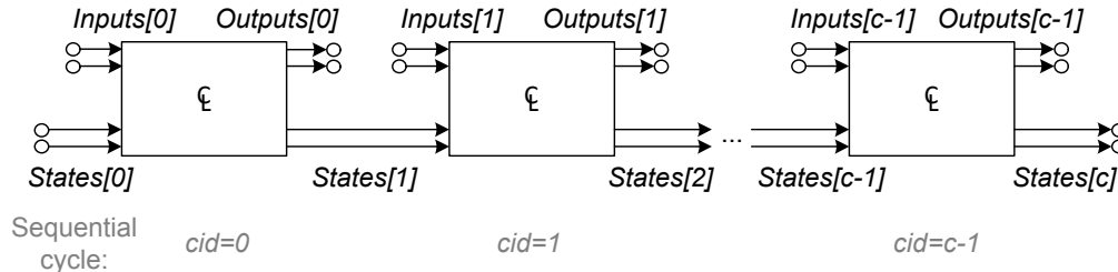
Fig. 5: Functionally equivalent unrolled sequential circuit corresponding to Fig. 3b.
