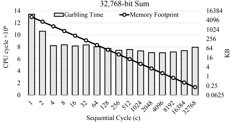
Fig. 7: Garbling 32,768-bit Sum function. The CPU time in number of cycles and the approximate memory footprint in KBytes (y-axis) versus c (x-axis) are shown.
