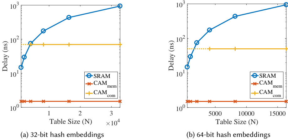
Fig. 6. Delay analysis for hash embeddings of size 32 and 64-bit. CAM_{mem} and CAM_{com} denote memristive and commercial CMOS-based CAMs, respectively. The dotted line for CAM_{com} shows interpolated data.
