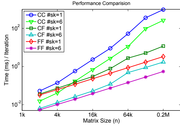
Fig. 5: Time per iteration for solver implementations with different number of Solver Kernels versus size of data is shown. CC method directly uses \mathbf{A} , while CF and FF leverage the learned decomposed matrices ( \mathbf{D} and \mathbf{V} ).
